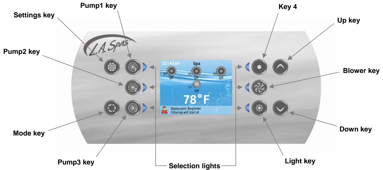
in.k806 Control Panel
